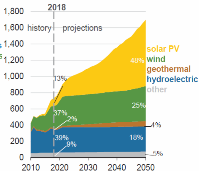
Renewable electricity generation, including end-use (Reference case)
